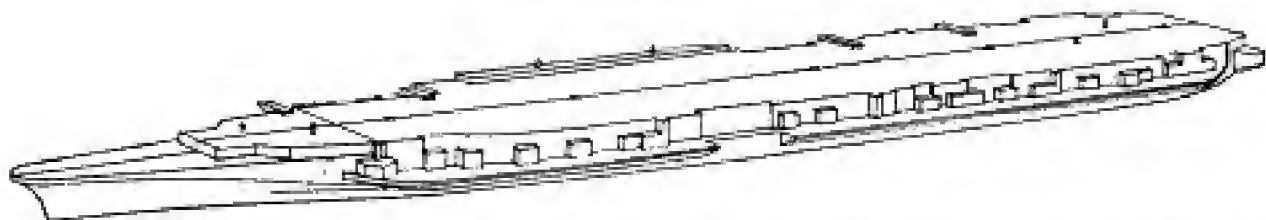
Portside view of hull shows sponson, notched piece, island base, forecastle, tower bases and stern bumpkins
